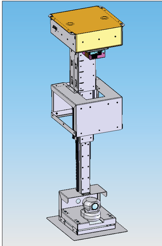
*Plenum housing removed for clarity.
